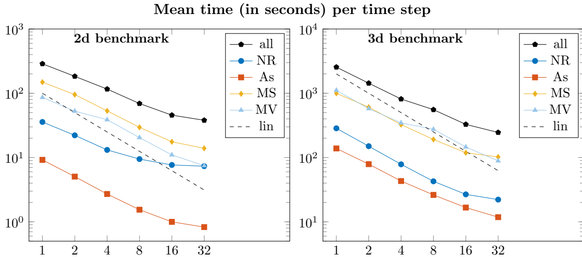
Figure 7: Strong scalability test. Mean time per timestep (all) to compute the Newton residual (NR), assemble the Jacobian (As), multilevelsolver (MS), matrix-vector multiplication (MV) in 2d (left) and 3d (right) using 1-32 threads on mesh levels 6 and 3.
