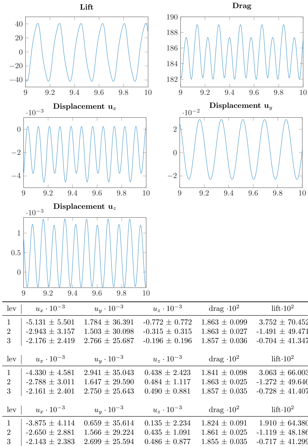
Figure 3: 3d fsi-3 configuration. Top: functional values as function over the time interval I = [9, 10] for k = 0.001s and mesh level 3. Bottom: results for time step sizes k = 0.004s , k = 0.002s , k = 0.001s and all three mesh levels.
