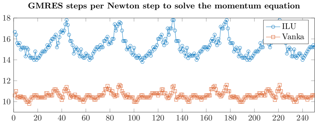
Figure 5: 3d fsi-3 configuration: Mean number of GMRES steps to solve the momentum equation (9) within every Newton step plotted over time steps
