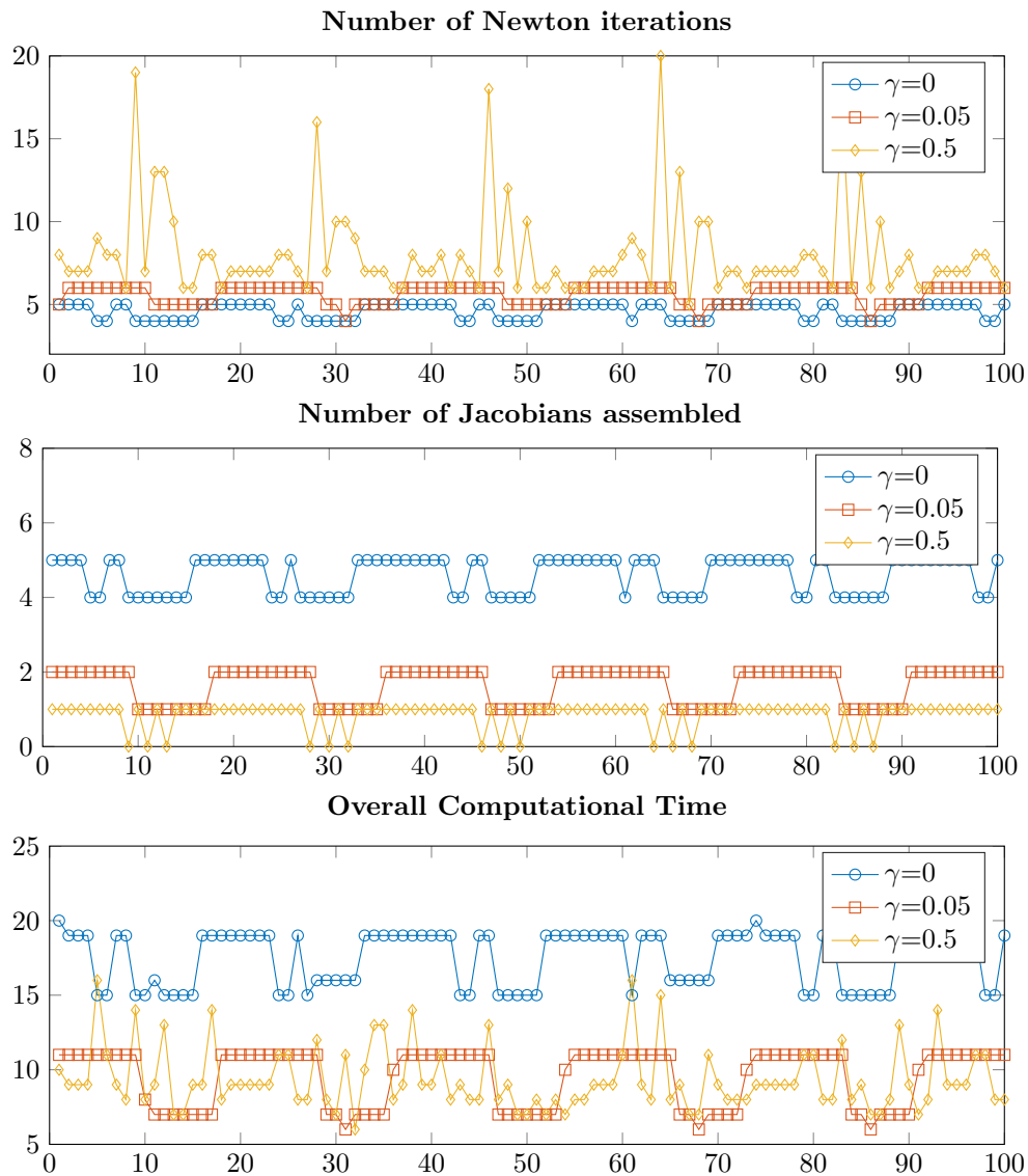
Figure 2: Study on the effect of the non-exact Newton scheme for the 2d benchmark problem. The Jacobian is only reassembled, if the Newton rate is above \gamma . Top: number of Newton iterations per time step. Middle: Number of Jacobians assembled in each time step. Bottom: overall computational time in each time step.
