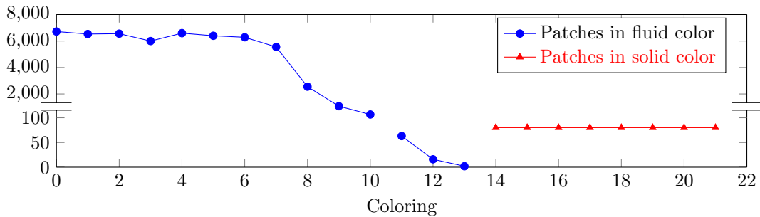
Figure 6: Coloring for avoiding memory collisions in the parallel Vanka smoother for the finest 3d mesh with about 3.5 \cdot 10^6 dofs. The fluid patches consist of 108 dofs each, while the solid patches couple 500 dofs. The smallest fluid color has only 2 patches.
