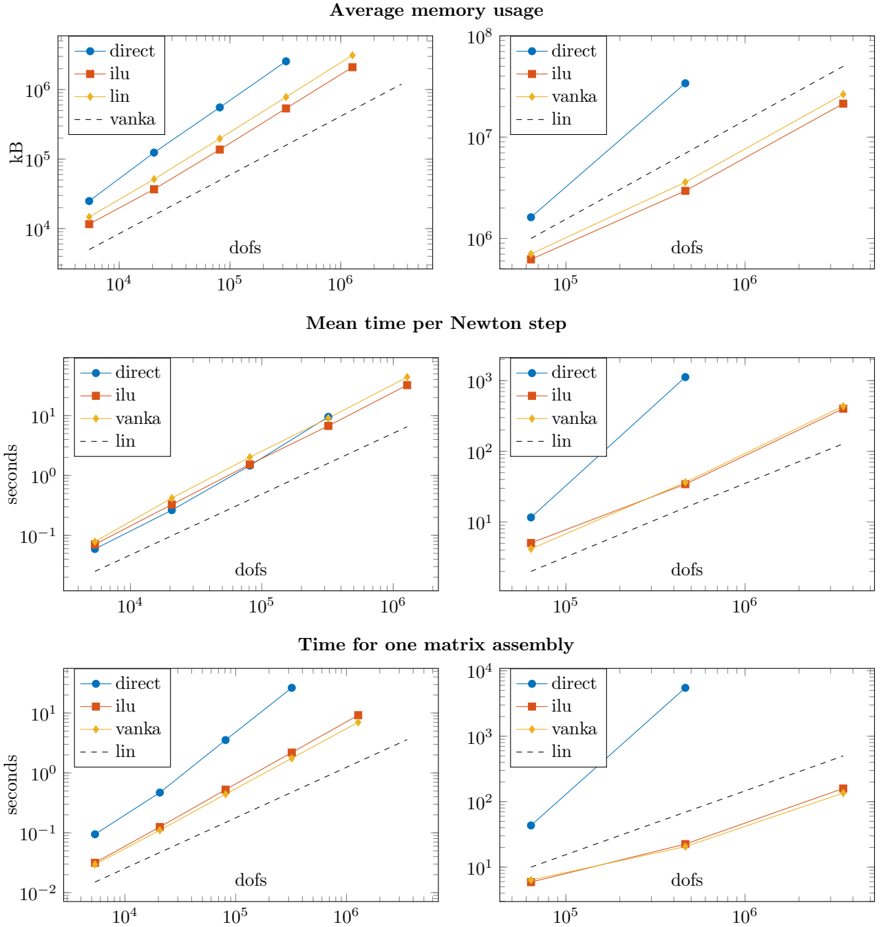
Figure 4: Performance of the multigrid solver in 2d (left) and 3d (right) in comparison to a direct solver. On different meshes with increasing numbers of degrees of freedom, we compare the performance of the direct solver UMFPACK [12] with the multigrid solver based on ILU smoothing and based on Vanka smoothing. No parallelization is employed. From top to bottom: average memory usage, average time per Newton step and time to assemble one system matrix including preparation of the direct solver and the smoothers. Note that we do not reassemble the Jacobian in every Newton step, and therefore, assembly times can be higher than mean Newton times (which include the assembly).
