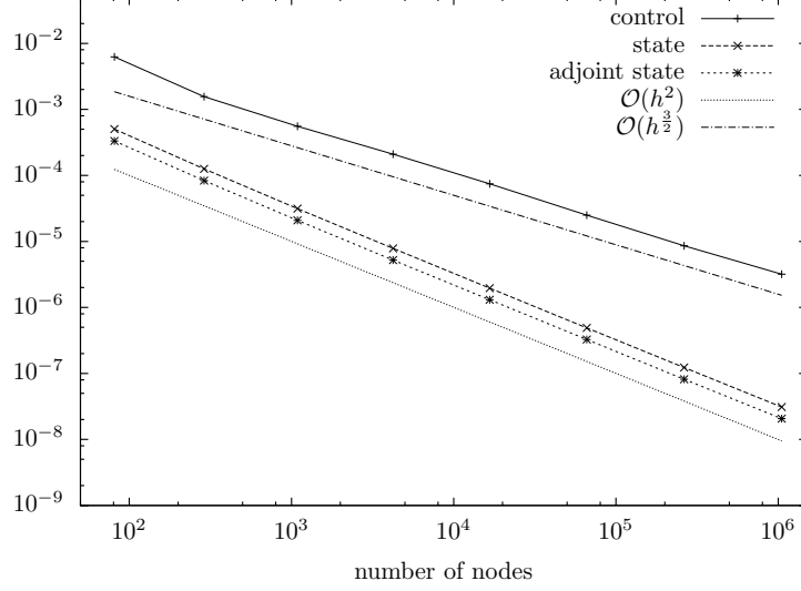
Figure 3: Example 6.2: Discretization error of the control, state and adjoint state when discretizing the control by continuous cellwise bilinear finite elements
