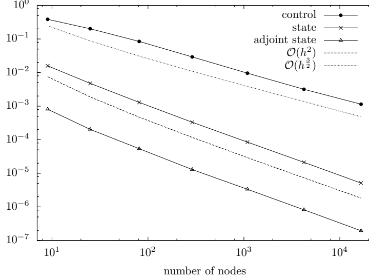
Figure 2: Example 6.1: Discretization error of the control, state and adjoint state when discretizing the control by continuous cellwise bilinear finite elements
