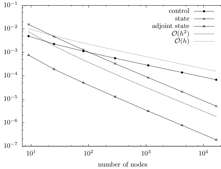
Figure 1: Example 6.1: Discretization error of the control, state and adjoint state when discretizing the control by cellwise constants
