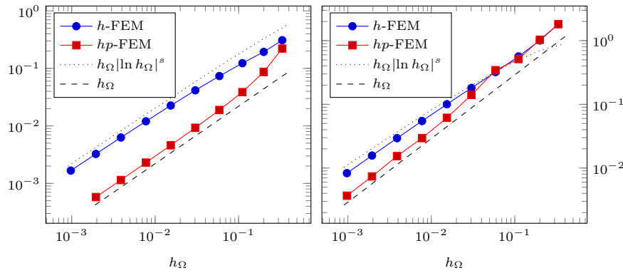
FIG. 1. \|y^{\frac{s}{2}} \nabla(u - u_h)\|_{L^2(C)} for s = 0.2 (left) and s = 0.8 (right) over h_\Omega .
