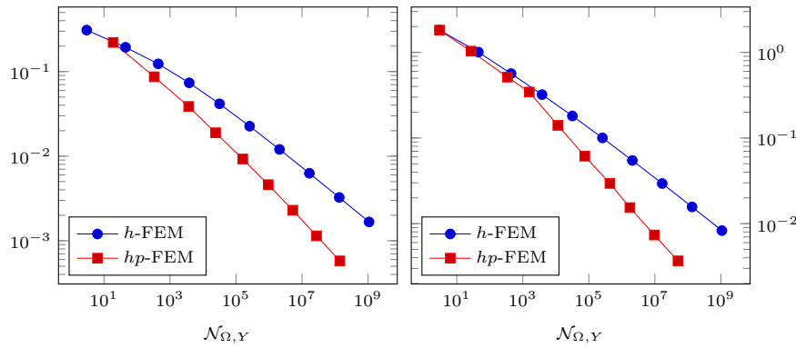
FIG. 2. \|y^{\frac{s}{2}} \nabla(u - u_h)\|_{L^2(C)} for s = 0.2 (left) and s = 0.8 (right) over the total number of degrees of freedom N_{\Omega,Y} .
